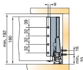
Tekform drawer DW145
